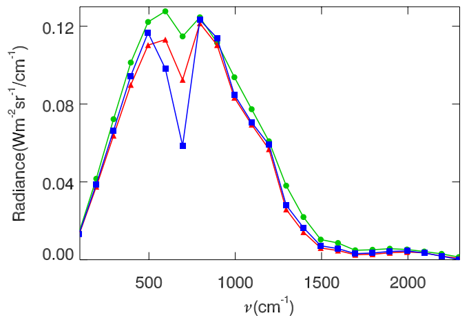
Fig. 4. The emission spectra of the Earth's atmosphere corresponding to the 3 stages shown in Fig. 3. Blue: Stage A with 330 ppm \text{CO}_2 under 1 atmospheric pressure; red: Stage B with 10 ppm \text{CO}_2 under 1 atmospheric pressure; and, green: Stage C with 10 ppm \text{CO}_2 under 0.08 atmospheric pressure.
