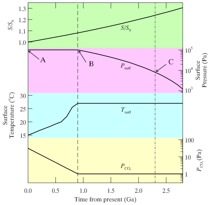
Fig. 3. The evolution of surface pressure and temperature and the partial pressure of \text{CO}_2 in the model as the solar luminosity evolves in the next 2.8 Ga from present. Before 0.9 Ga (dashed line), the quantities evolve as described in Caldeira and Kasting (8). After 0.9 Ga, the surface temperature and the partial pressure of \text{CO}_2 at the surface ( P_{\text{CO}_2} ) are kept constant while the atmospheric pressure is lowered to compensate the temperature increase due to the increase in solar luminosity (see Models and Results ). At \approx 2.3 Ga (dash-dotted line), runaway greenhouse occurs, signaling the ultimate fate of the biosphere.
